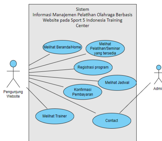
Figure 1. Software implementation
