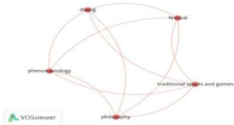
Figure 3. VOSviewer
